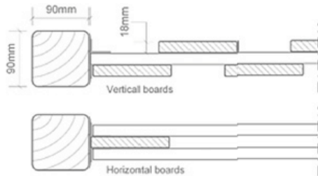
Shadow box, cross section
