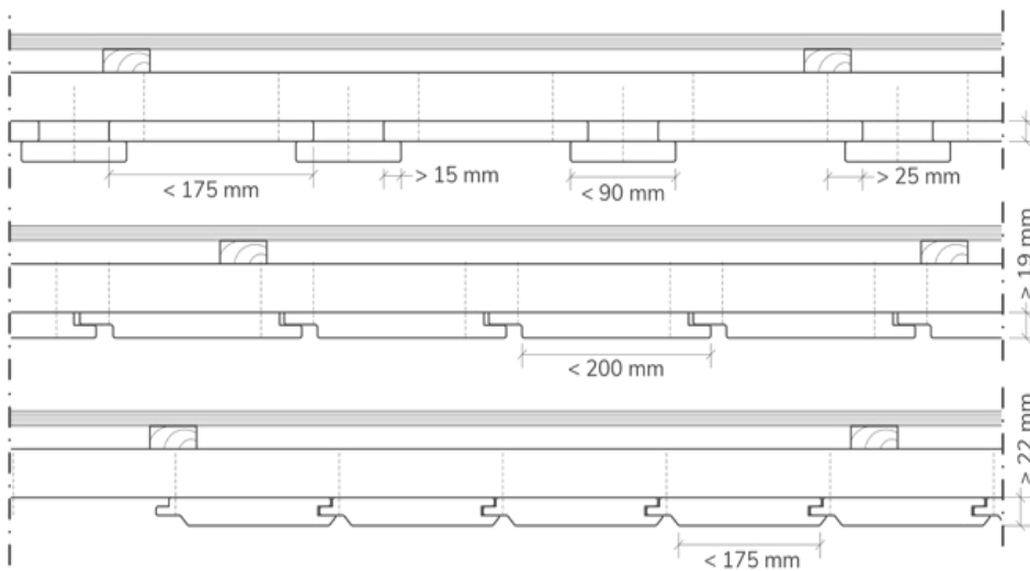
Profiles and dimensions for vertical cladding
