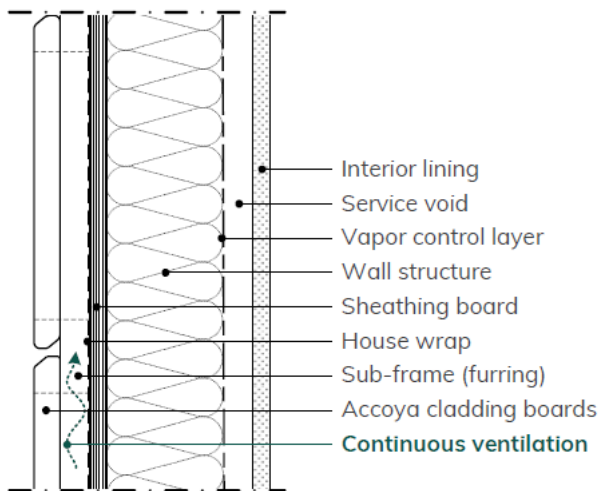
Ventilated Cladding system
