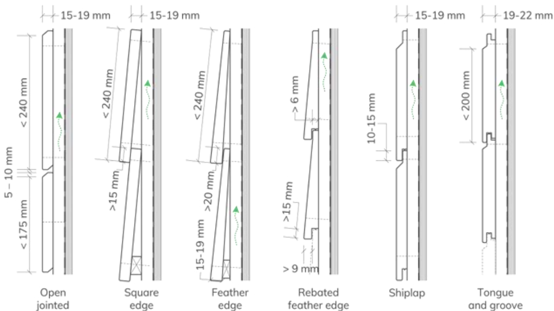
Profiles and dimensions for horizontal cladding
